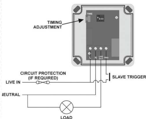
Diagram 1 Standard Wiring
