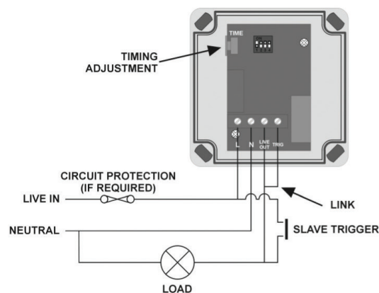
Diagram 2 Wiring for three wire switching circuits
