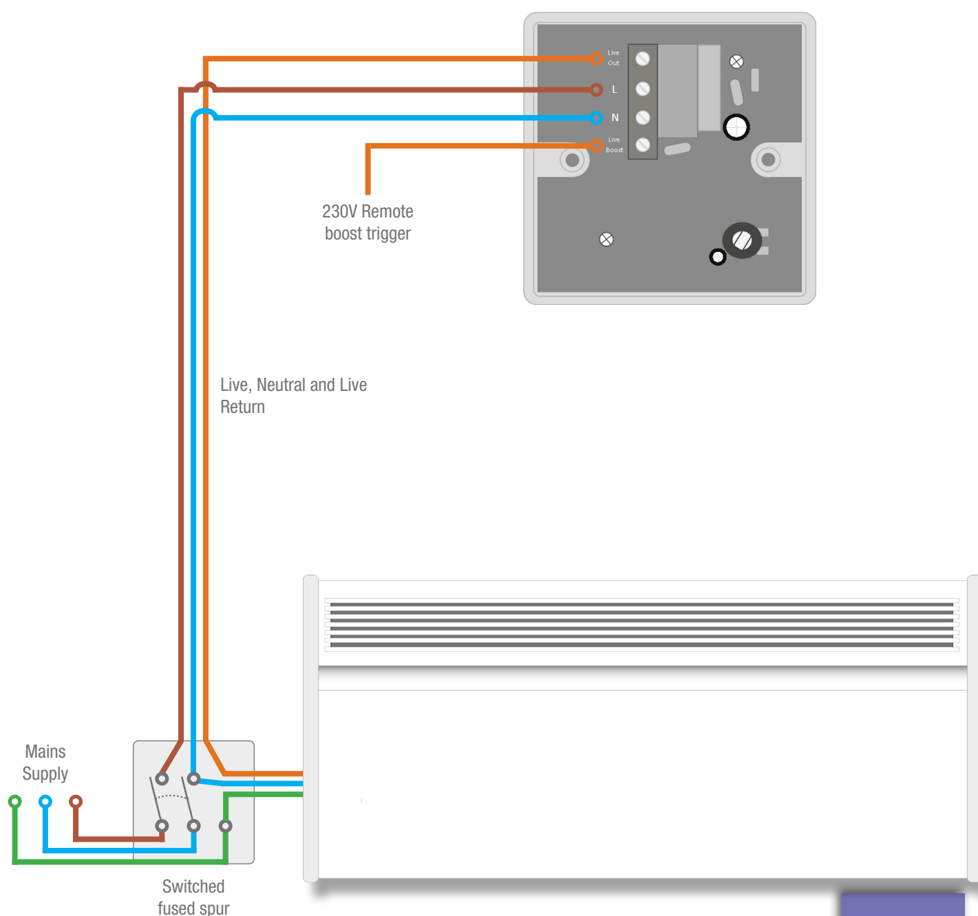
Rear view of Thermostat
